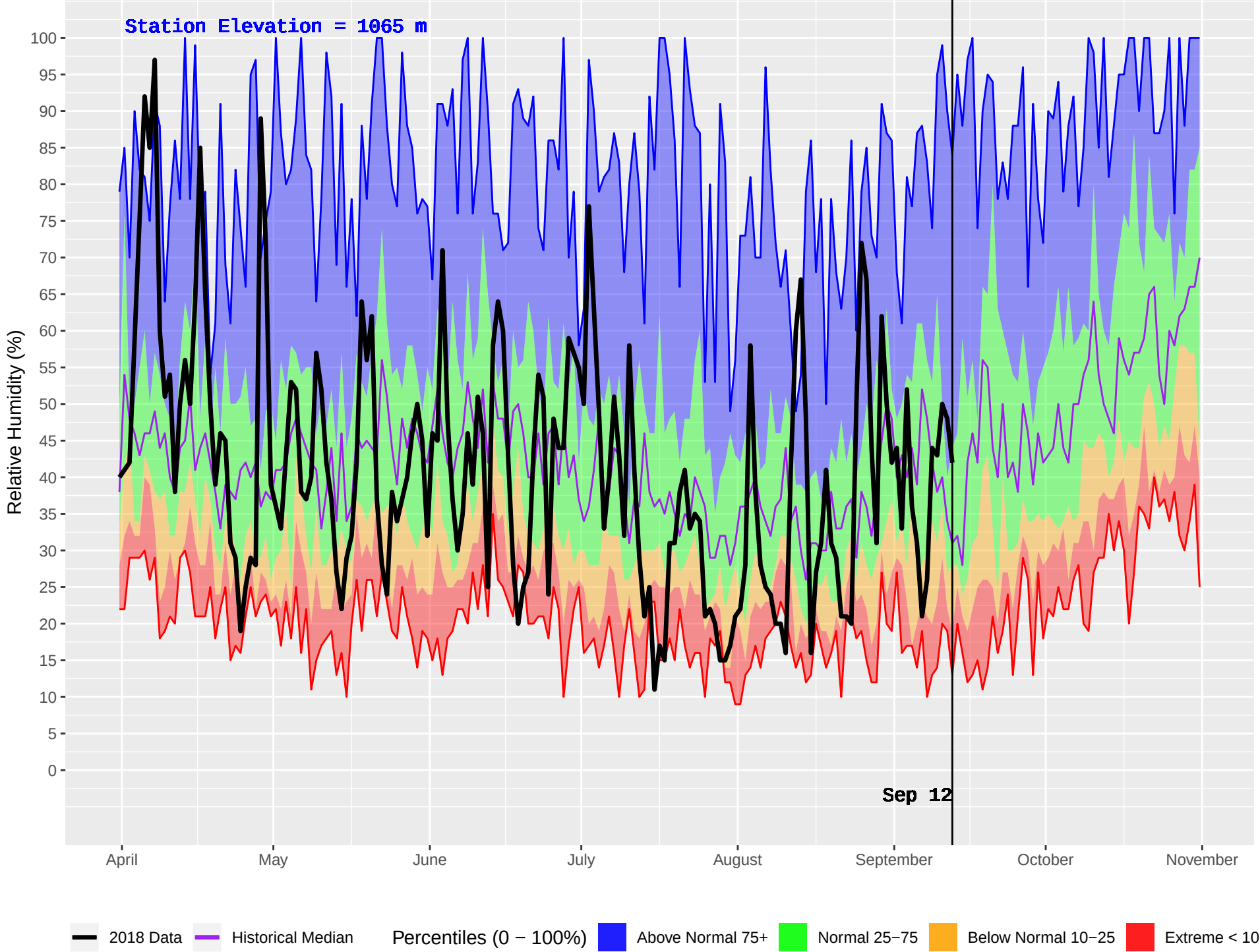
ASPEN GROVE (302) : Historical (1998–2016) and Current (2018) Daily Relative Humidity
