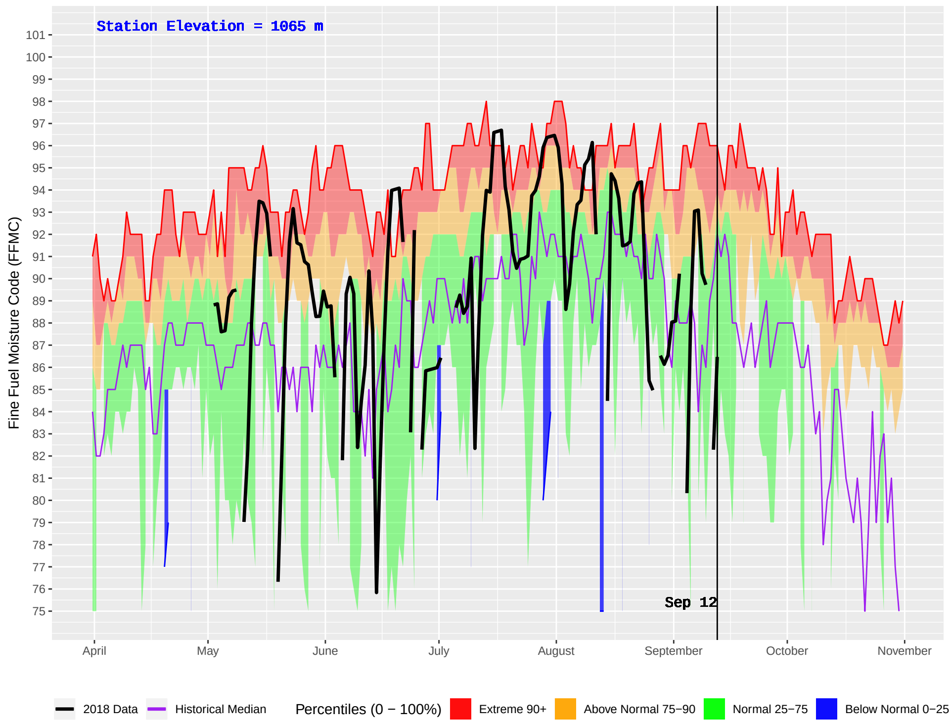
ASPEN GROVE (302) : Historical (1998–2016) and Current (2018) Daily Fine Fuel Moisture Code (FFMC)
