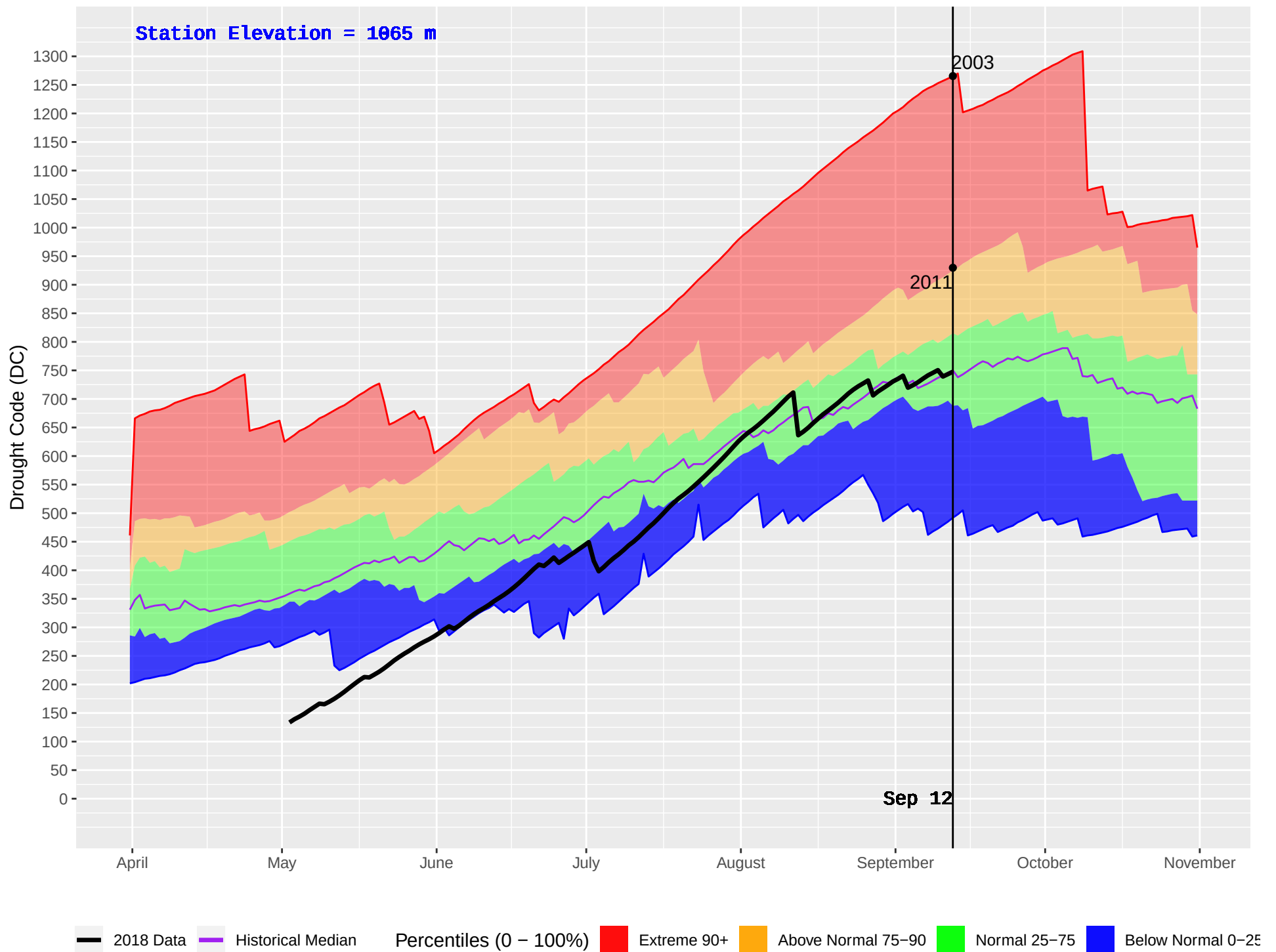
ASPEN GROVE (302) : Historical (1998–2016) and Current (2018) Daily Drought Code (DC)
