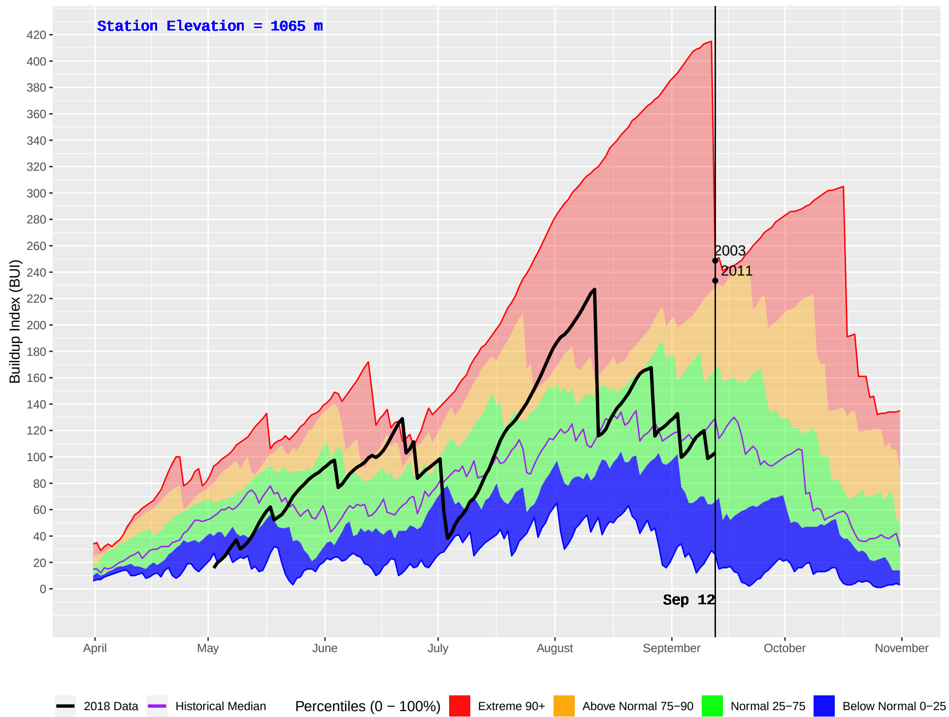
ASPEN GROVE (302) : Historical (1998–2016) and Current (2018) Daily Buildup Index (BUI)
