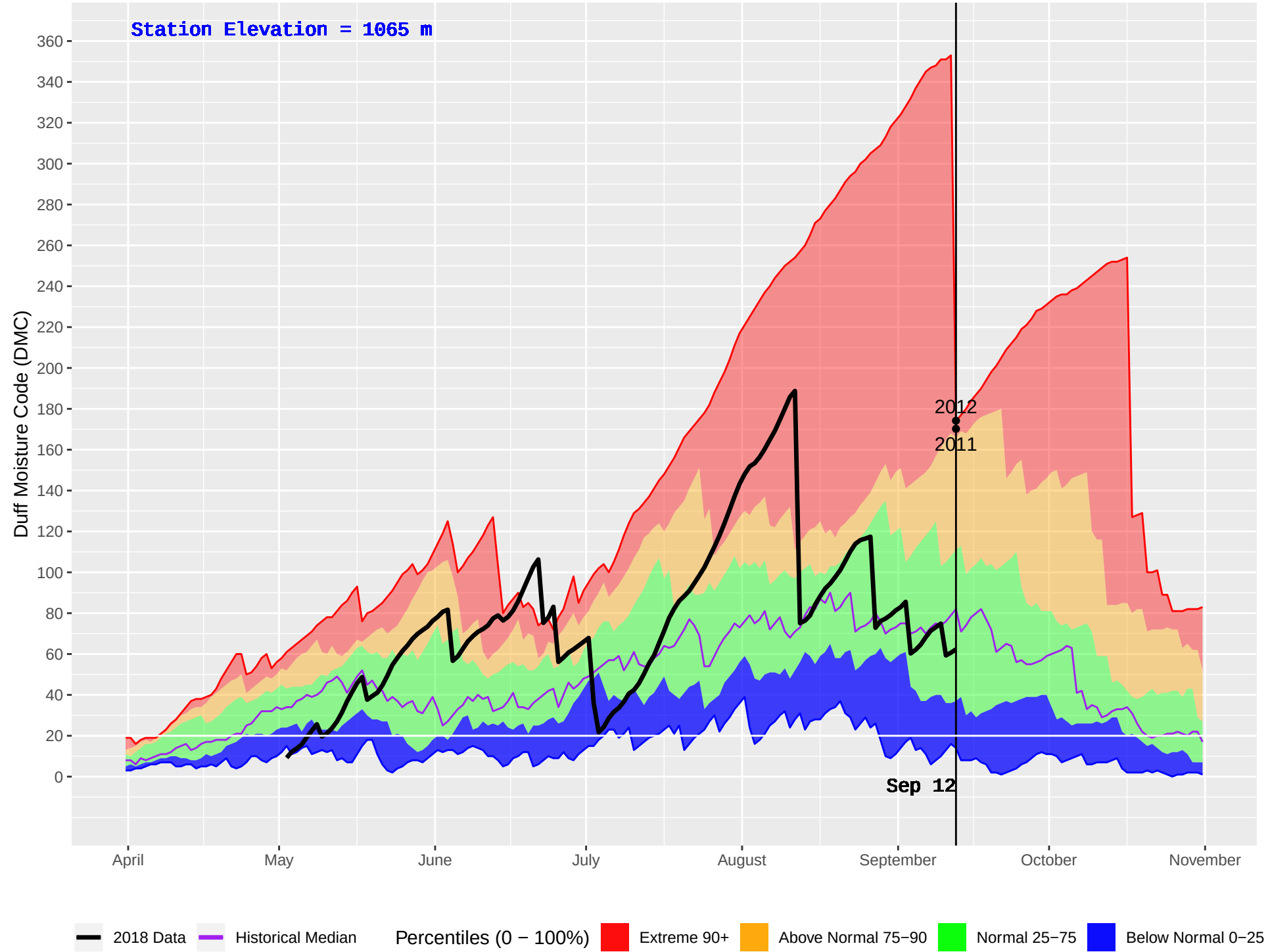
ASPEN GROVE (302) : Historical (1998–2016) and Current (2018) Daily Duff Moisture Code (DMC)
