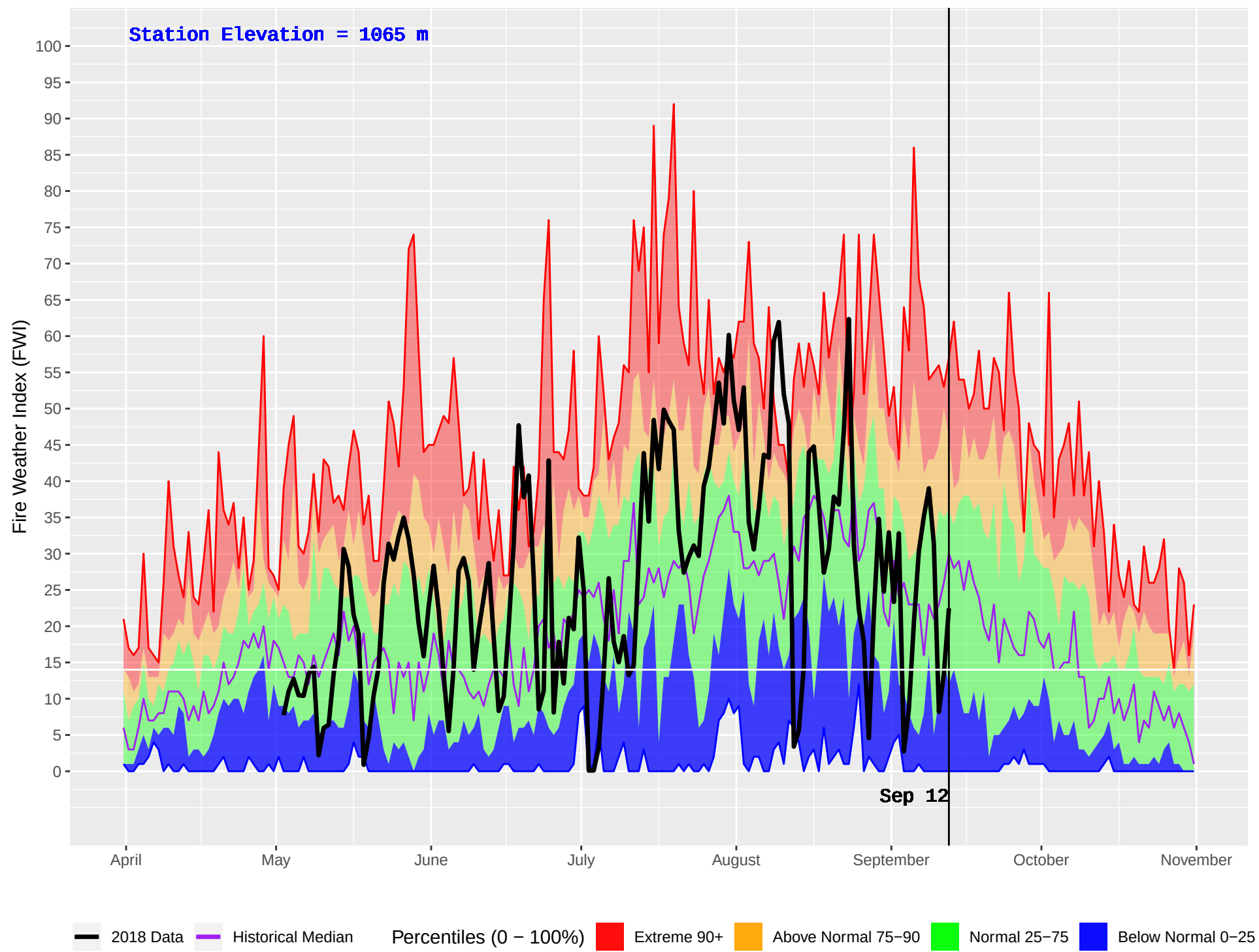
ASPEN GROVE (302) : Historical (1998–2016) and Current (2018) Daily Fire Weather Index (FWI)
