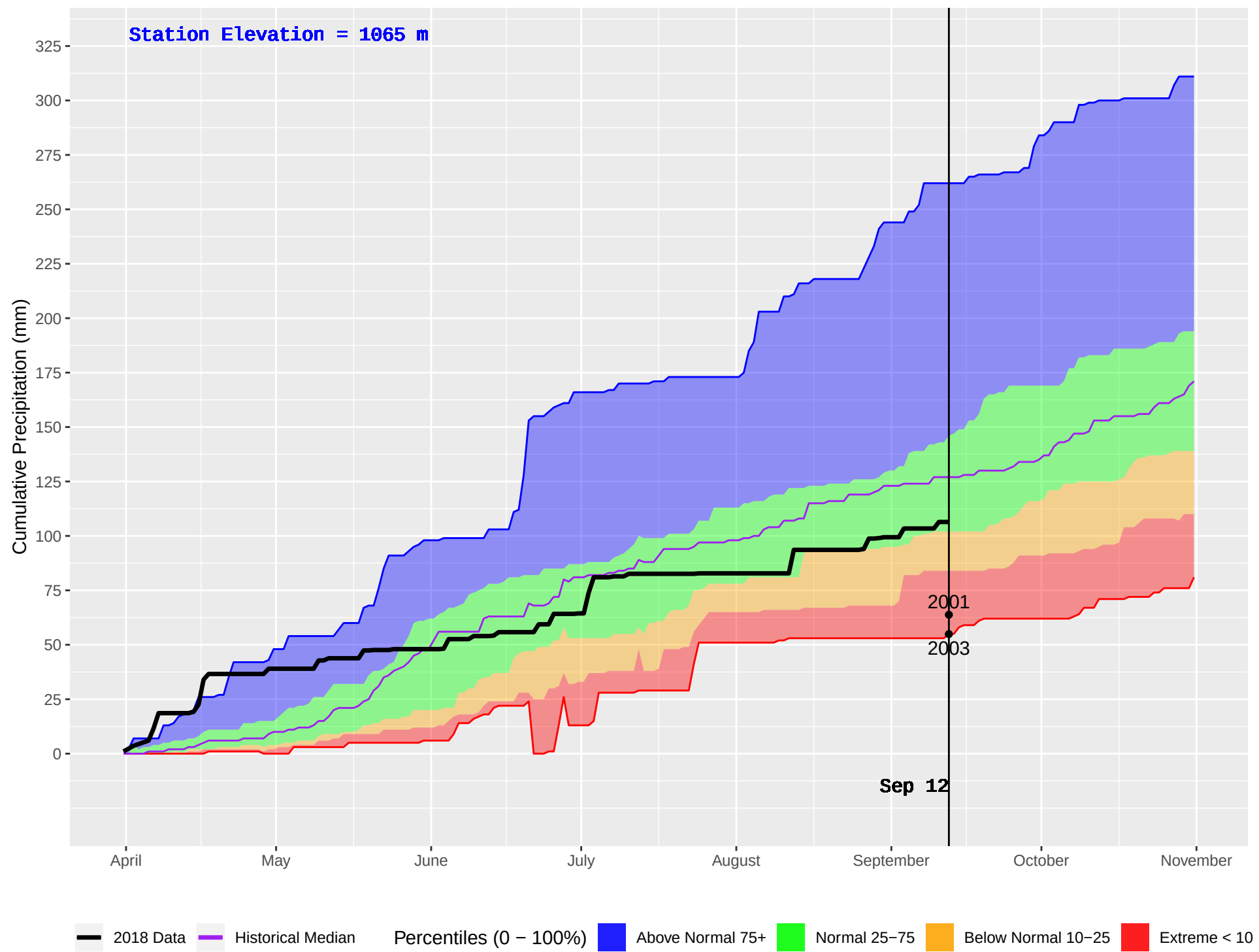
ASPEN GROVE (302) : Historical (1998–2016) and Current (2018) Daily Cumulative Precipitation
